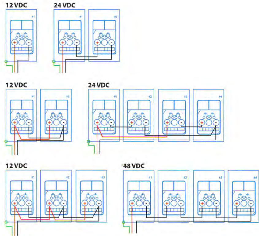
PV Panel Wiring (bottom view)
