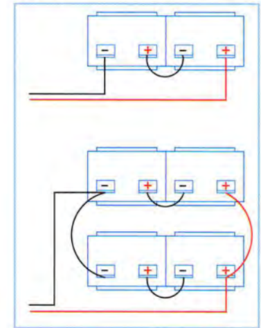
48 VDC
