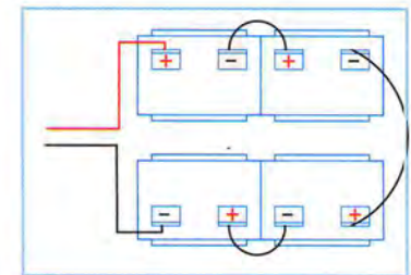
48 VDC
