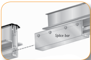
Splice Bar
