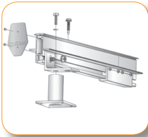
SunFrame components
