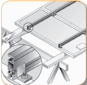
SolarMount Bottom Up Mount
