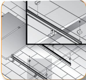
SolarMount Top Down Mount
