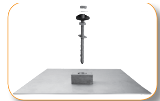
Quick Mount assembly
